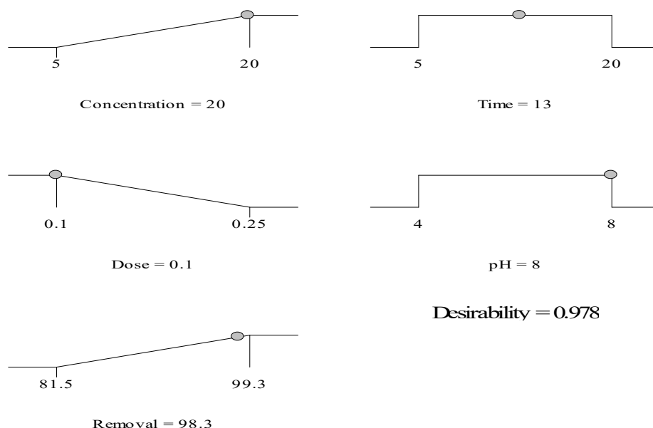
Fig.-2b: Desirability Ramp for Numerical Optimization
