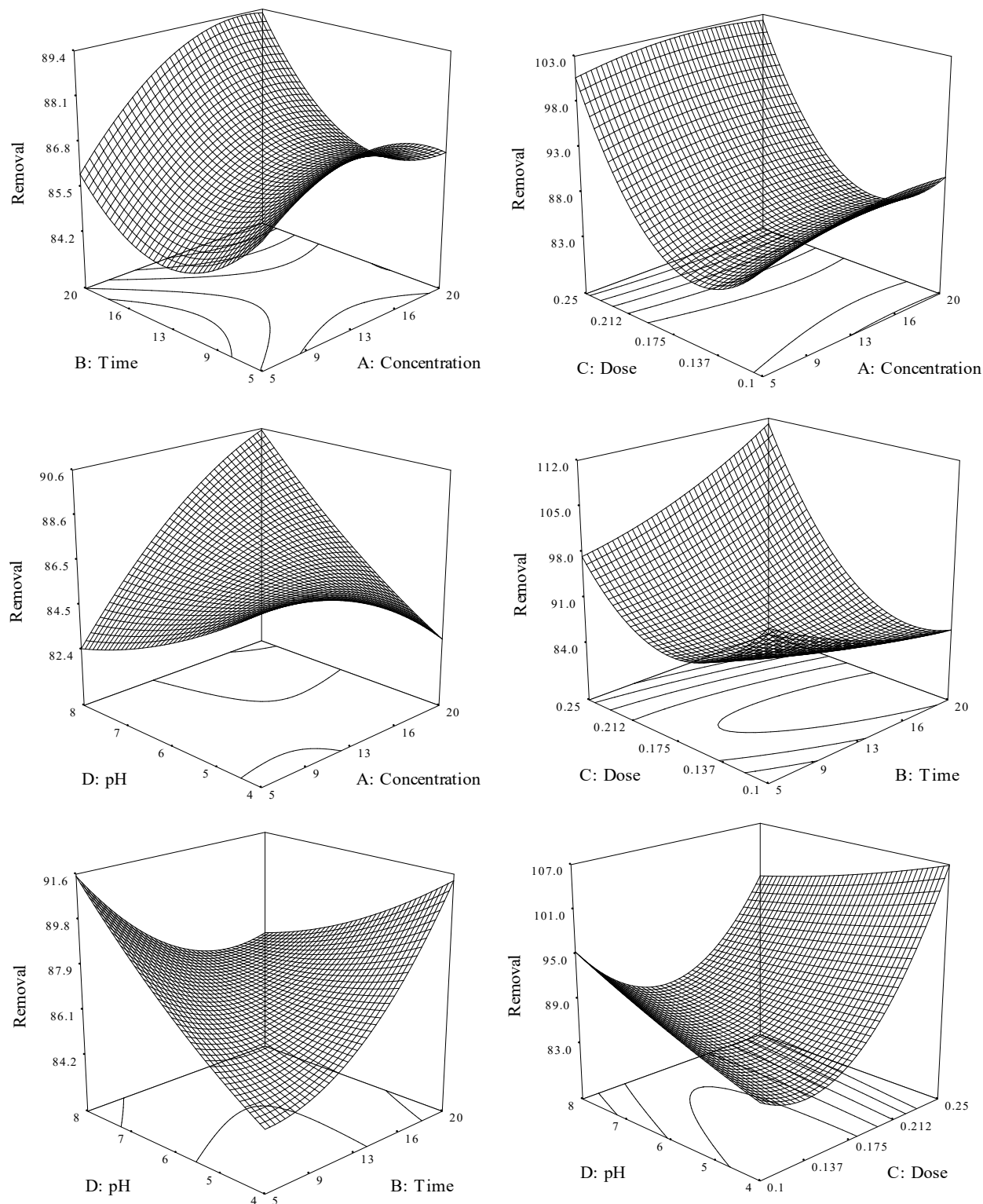
Fig-1: Response Surface Plots Showing the Effect of Tested Variables on Cr(VI) Removal by Fe-SCC
