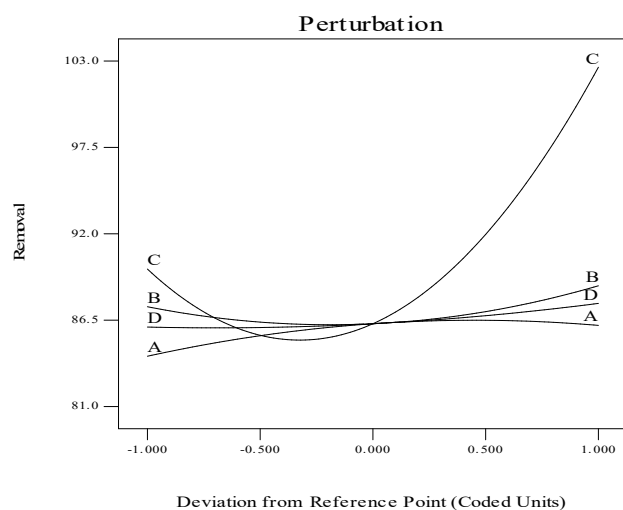
Fig.-4: Perturbation Plot Showing The Effect of Tested Variables
