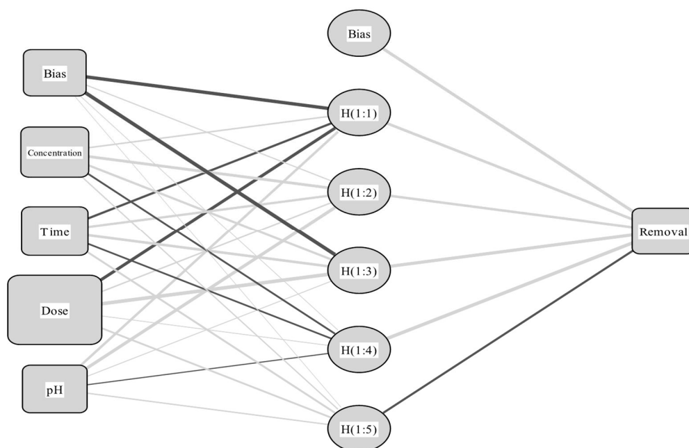
Fig.-3: Neural Network Architecture of Cr(VI)
