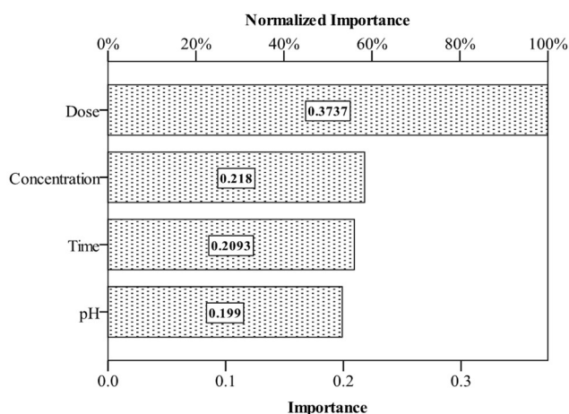
Fig.-5: Importance Analysis of Experimental (input) Parameters
