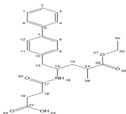
Sacubitril Chemical Formula: C_{24}H_{29}NO_5 Exact Mass: 411.20 Fig.-5a
