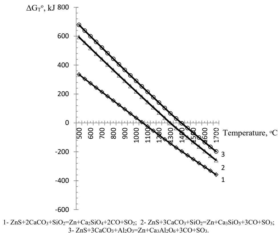
Fig.-1: Influence of Temperature on the Gibbs Energy of Formation of the Main Minerals of Cement Clinker in the Presence of Zinc Sulfide with Simultaneous Stripping of Zinc
